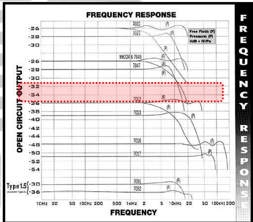
< Test Microphone Freq. Response >
